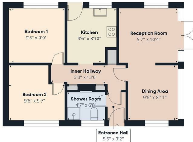
Floor 0 Building 1
